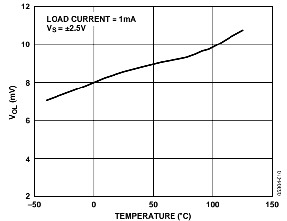
Figure 15. Output Voltage Swing Low vs. Temperature
