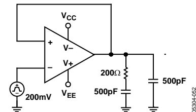
Figure 57. Snubber Network
