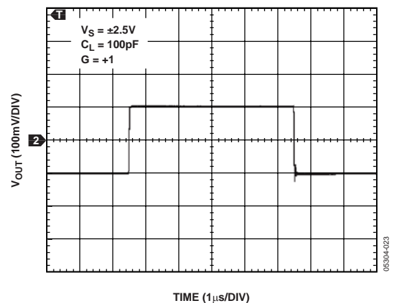
Figure 28. Small Signal Response
