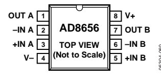
Figure 4. AD8656 8-Lead SOIC (R-8)
