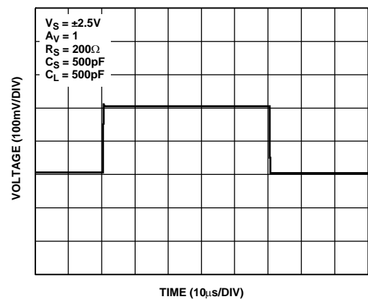
Figure 58. Driving Heavy Capacitive Loads Using a Snubber Network
