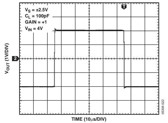
Figure 27. Large Signal Response
