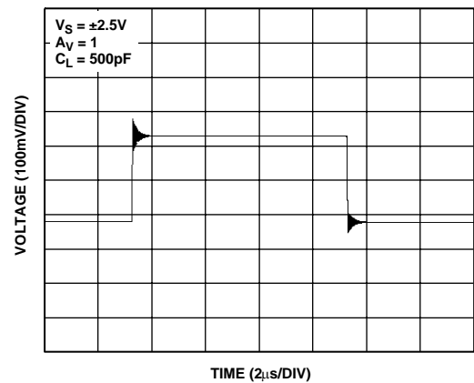
Figure 56. Driving Heavy Capacitive Loads Without Compensation
