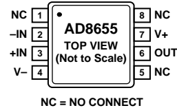
Figure 1. AD8655 8-Lead MSOP (RM-8)
