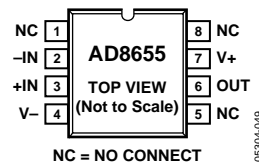
Figure 3. AD8655 8-Lead SOIC (R-8)
